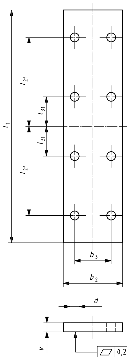
Figure 6 — Fishplate
